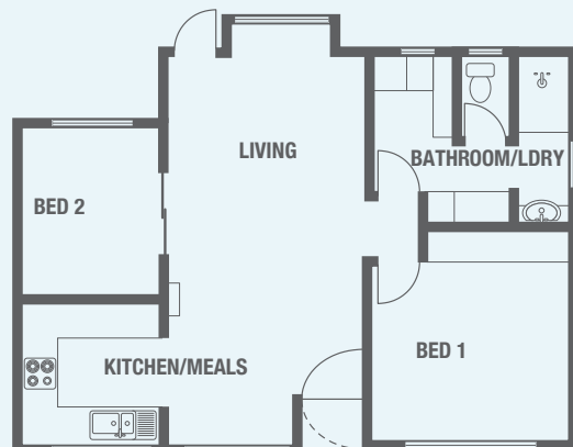
Two bedrooms, type 3
